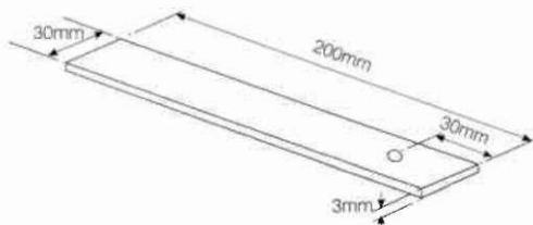
Fig. 1. "As supplied" test specimen.
