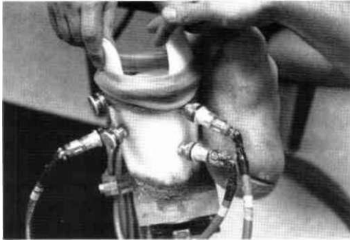
Fig. 1. An instrumented prosthetic socket. Transducers are positioned in mounts at anterior-medial proximal, antero-medial distal, lateral and posterior proximal sites. Dummy transducer plugs fill mounts at sites that are not monitored.
