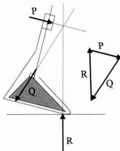
Fig. 7. Forces acting on AFO in late stance phase in the absence of plantar flexion power.
