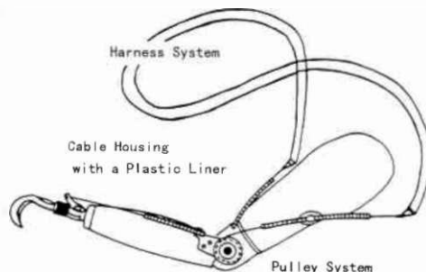
Fig. 1. Modified control cable system.
