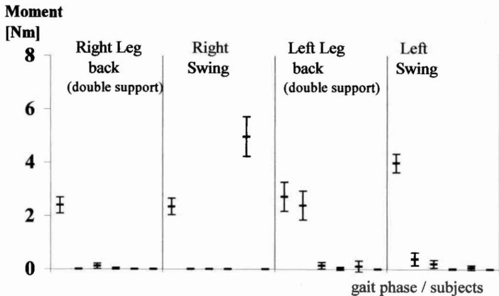
Fig. 7: Mean and standard deviation of the maximum hip moment produced by cable force in the front cable, grouped by gait phase, for all subjects. Within each phase subjects are shown in order (A-F).
