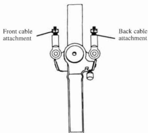
Fig. 2: Schematic representation of the hip joints and reciprocal cable link of an LSU-RGO.
