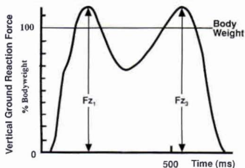
Fig. 1 shows a typical graph of the foot-ground reaction forces during normal gait. The two peak values ( Fz_1 and Fz_3 ) were compared in this study.
