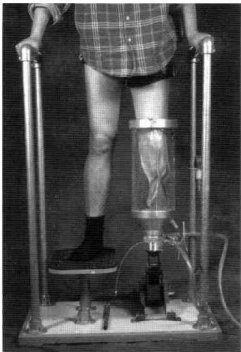
Fig. 1. Hydrostatic casting
