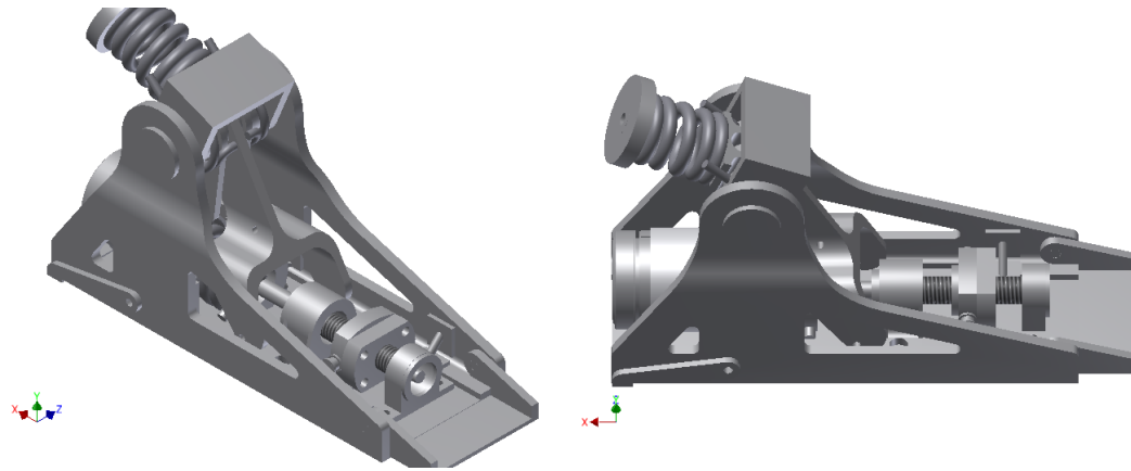
Figure 3.35: The prosthesis' arrangement at MDF. The leg is at 10^\circ and the small lever arm rotated over 15^\circ , compressing the spring positioned at the back of the prosthesis. The ball screw nut is still compressing the spring positioned over the motor axis.
