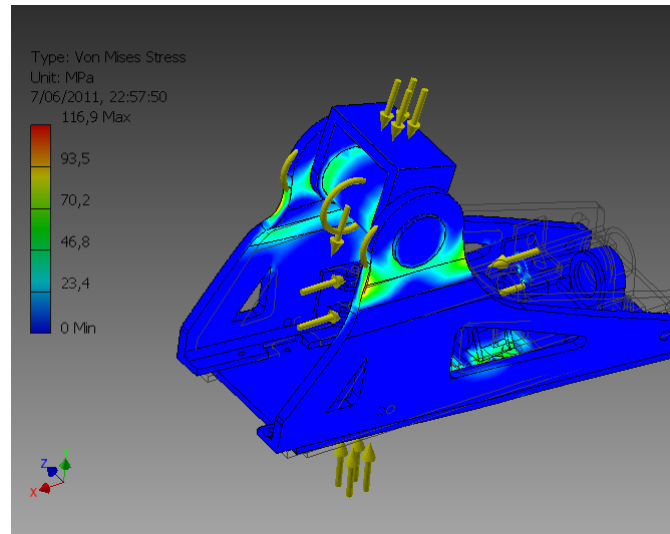
Figure 3.43: Load case 3 with a fixed constraint on the foot bottom plate.
