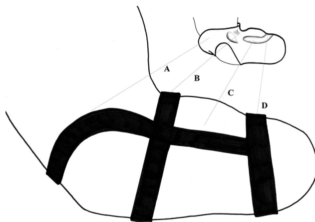
Figure 2. The ergonomic socket design conceptualized in 1985 was constructed of stainless steel tubes that were placed in anatomical regions to maximize the biomechanical efficiency of the design. These structural placements are similar to the region of anatomical consideration in the anatomical considerate transradial designs of today. A. Supra-condylar contour to promote medial-lateral and rotation stability. B. Ante-cubital/Supra-olecranon channel to enhance anterior-posterior stability. C. Wrist flexor/extensor channel to enhance weightbearing. D. Distal radial channel to allow weightbearing proximal to the cut end of the radius.
